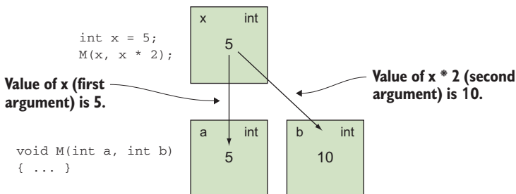
Figure 13.3 Calling a method with value parameters: the parameters are new variables that start with the values of the arguments.
