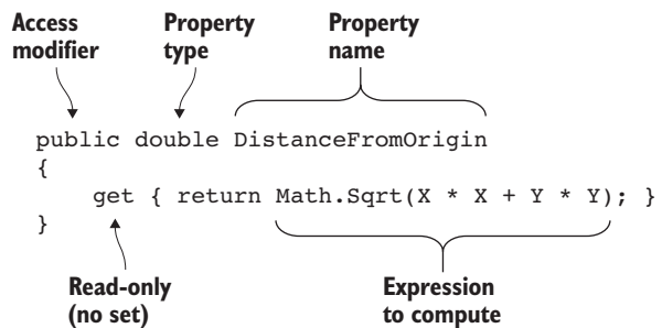
Figure 8.1 Annotated property declaration showing important aspects
