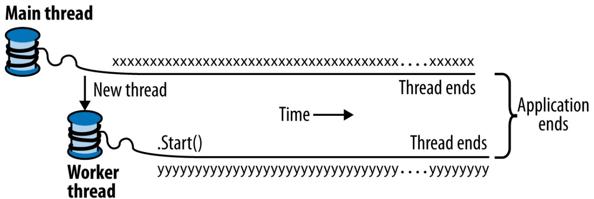
Figure 14-1. Starting a new thread
