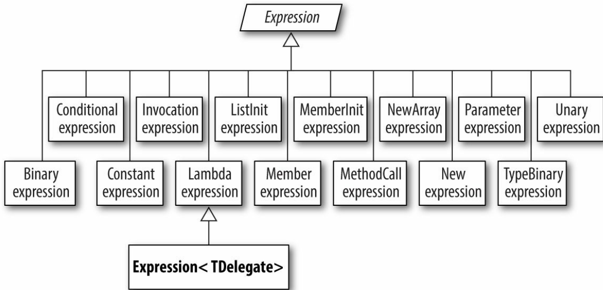
Figure 8-10. Expression types
