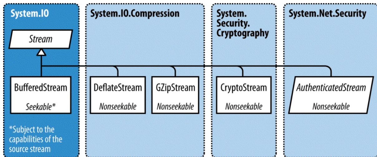
Figure 15-4. Decorator streams
