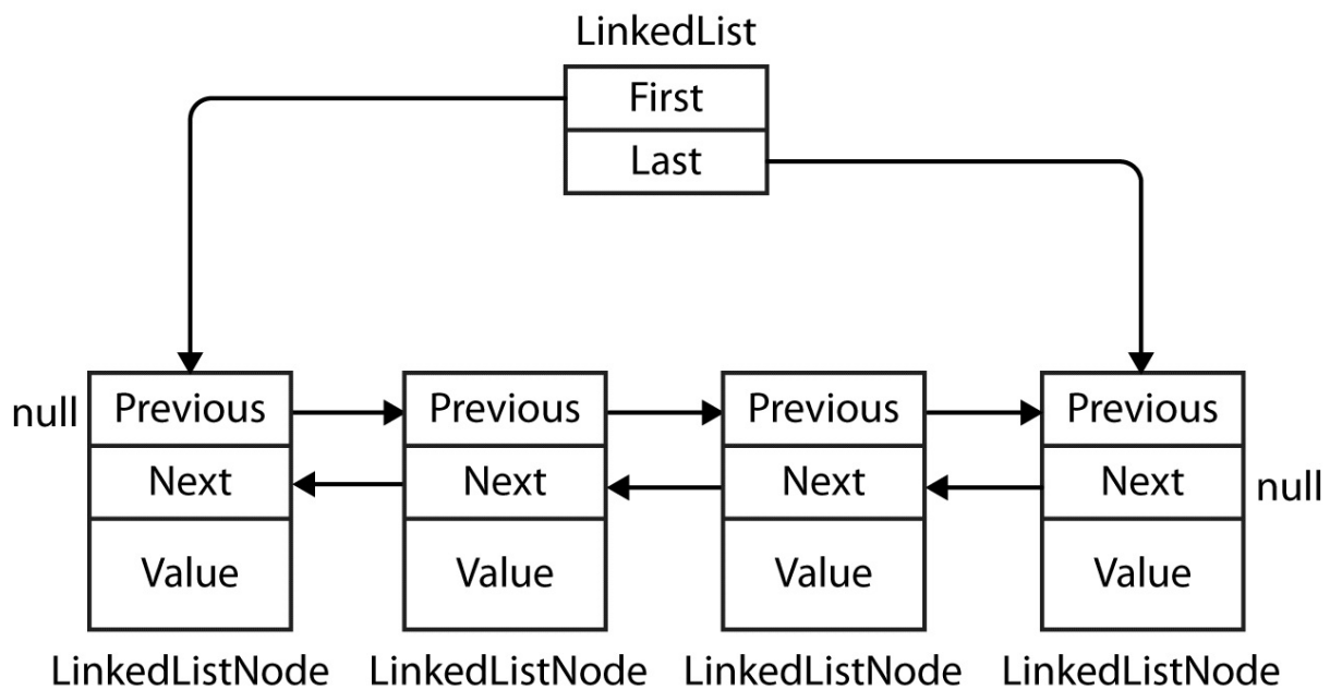
Figure 7-4. LinkedList<T>
