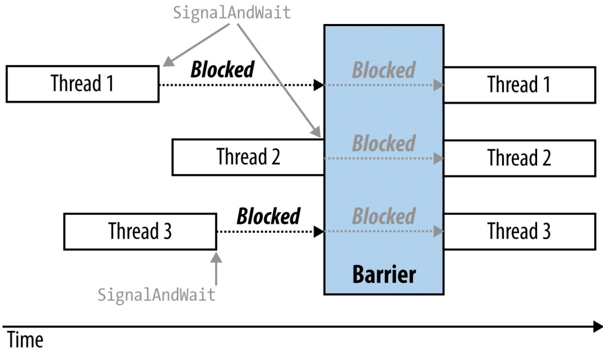
Figure 22-3. Barrier
