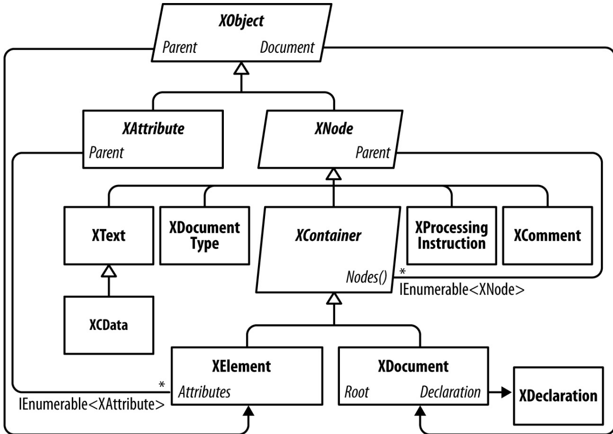
Figure 10-1. Core X-DOM types
