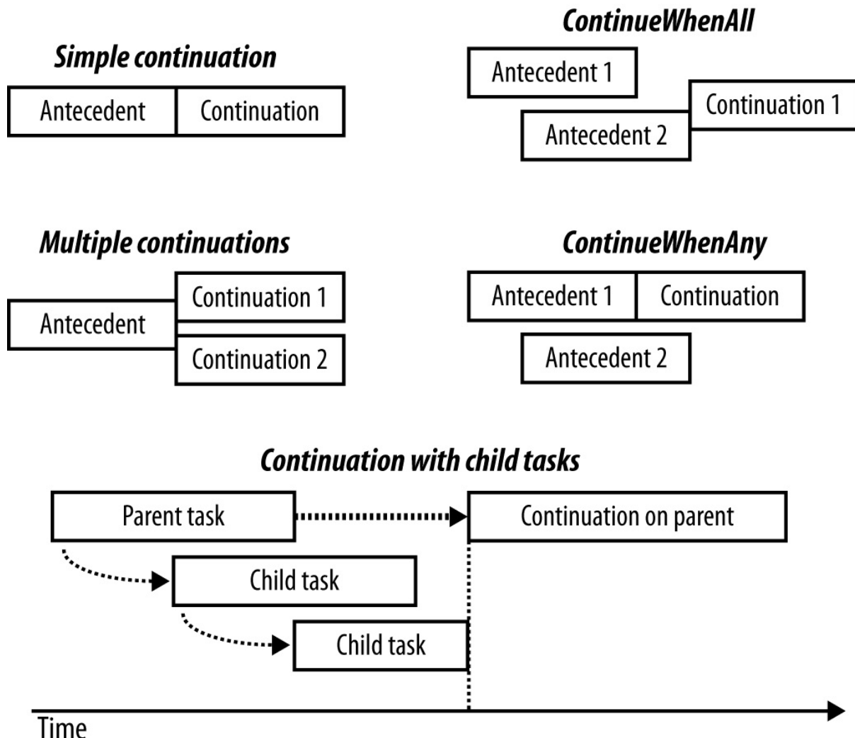
Figure 23-5. Continuations
