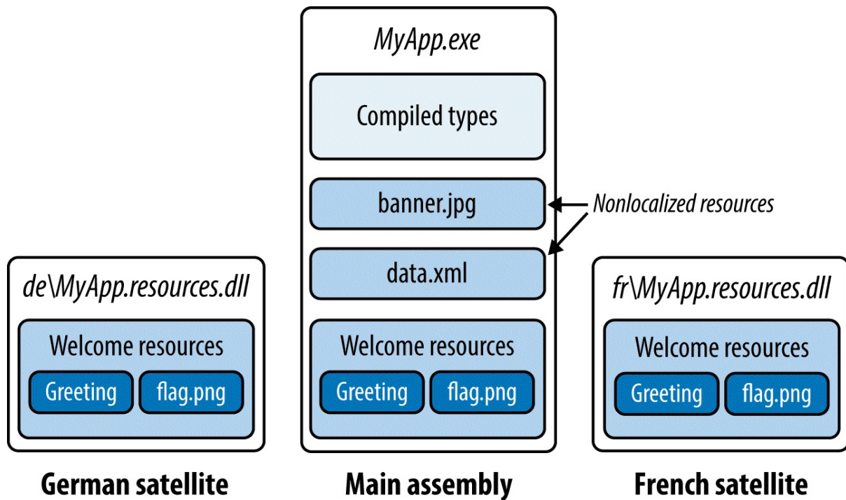
Figure 18-4. Resources
