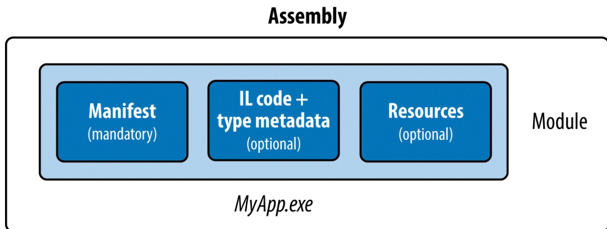
Figure 18-1. Single-file assembly
