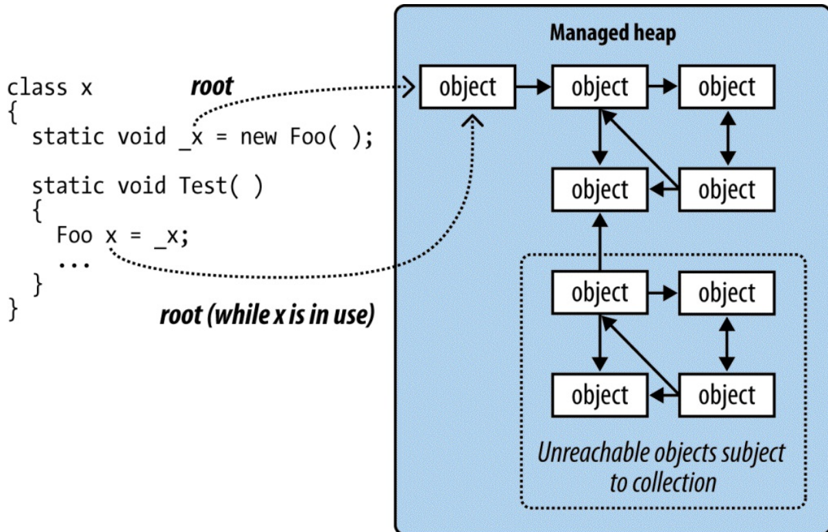
Figure 12-1. Roots
