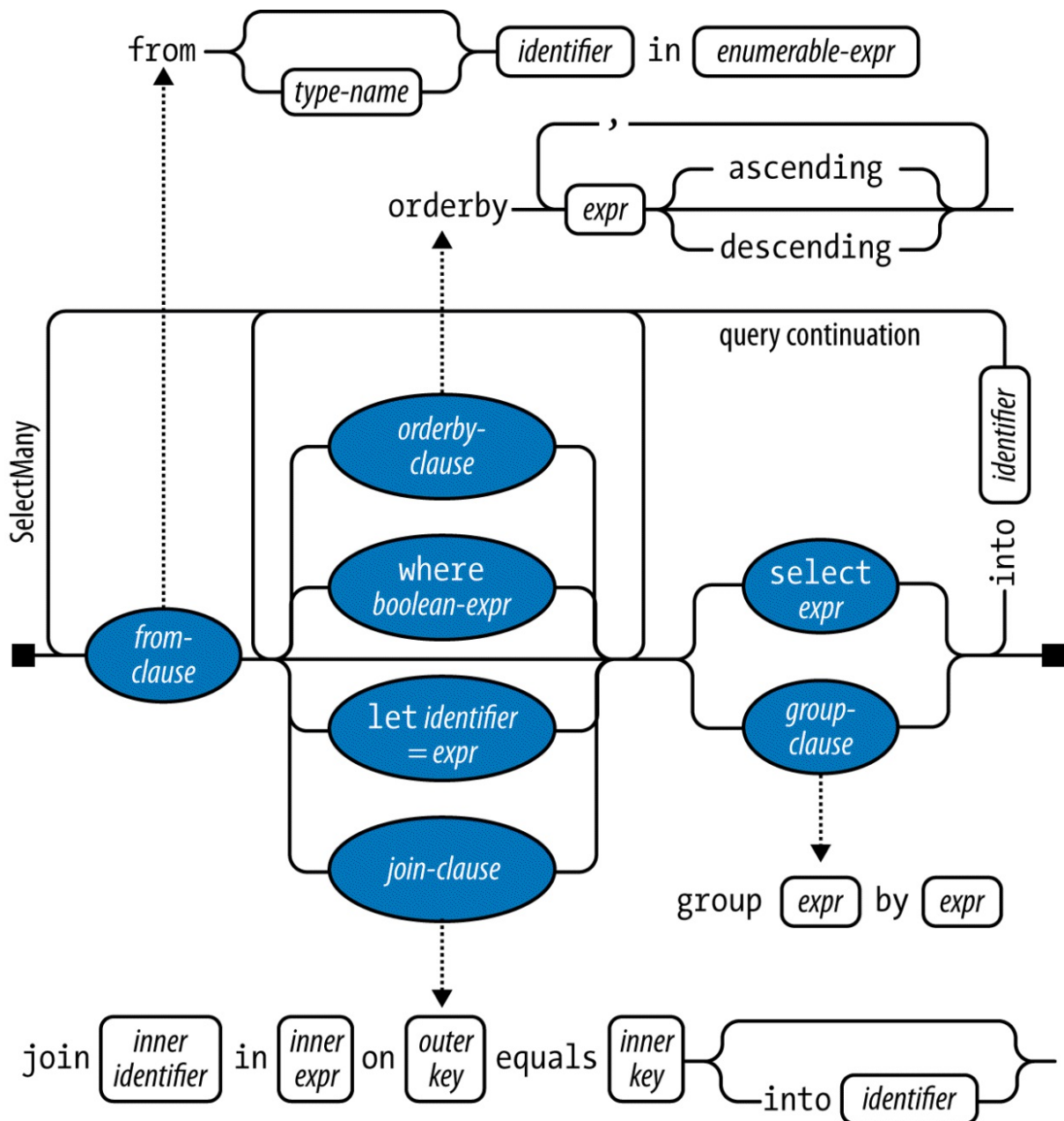
Figure 8-2. Query syntax
