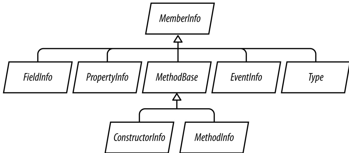
Figure 19-1. Member types
