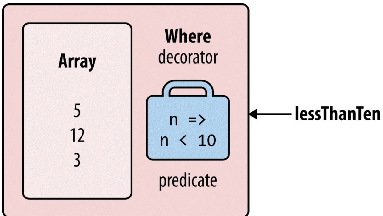
Figure 8-3. Decorator sequence
