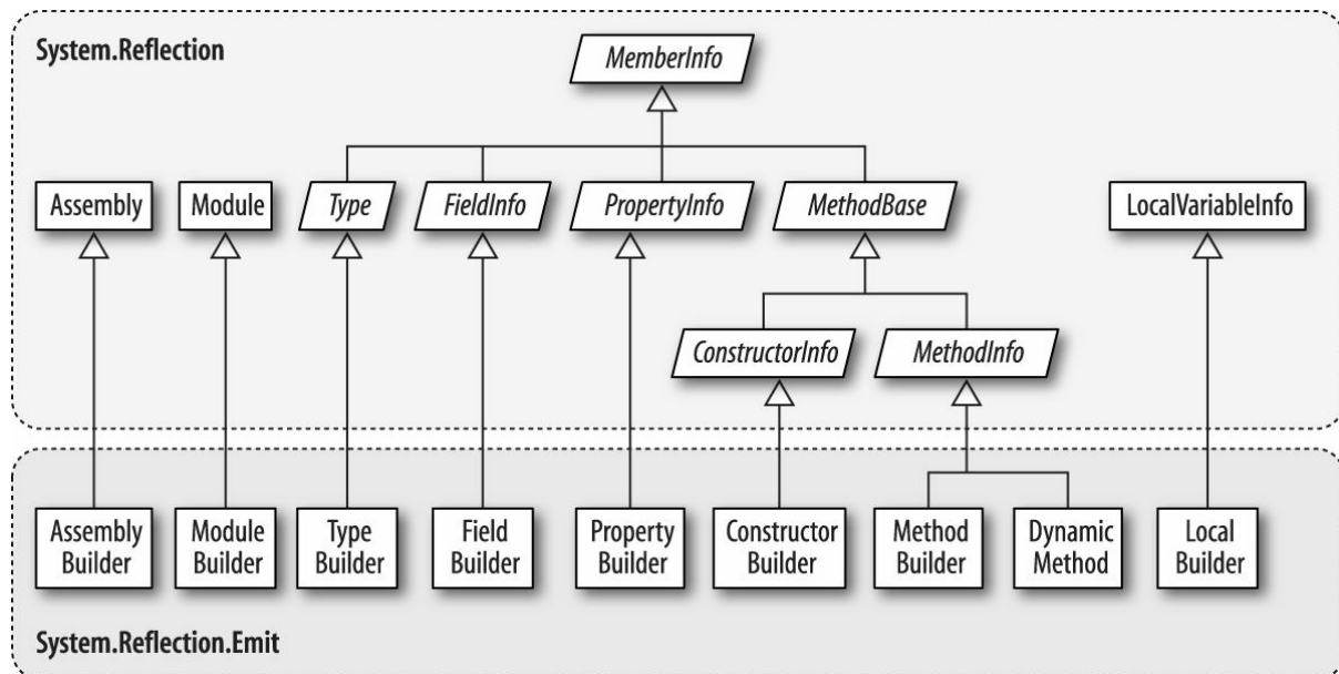
Figure 19-2. System.Reflection.Emit
