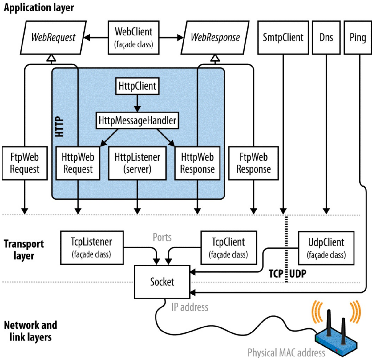
Figure 16-1. Network architecture
