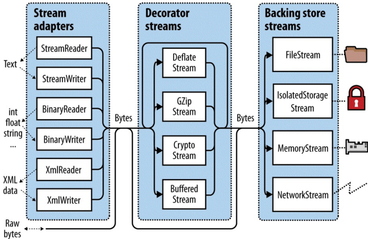
Figure 15-1. Stream architecture
