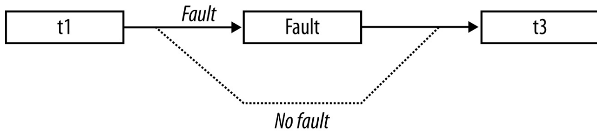
Figure 23-6. Conditional continuations
