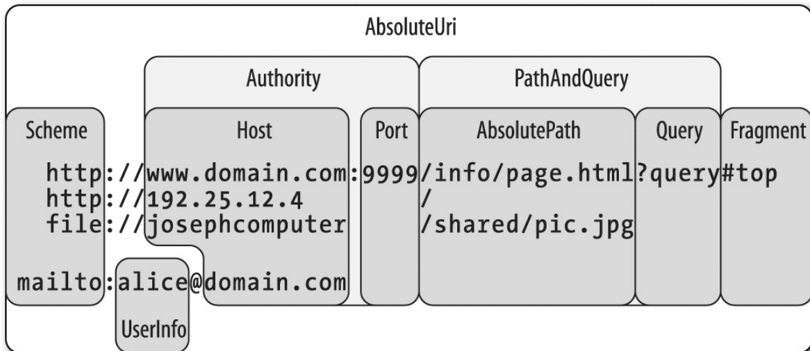
Figure 16-2. URI properties
