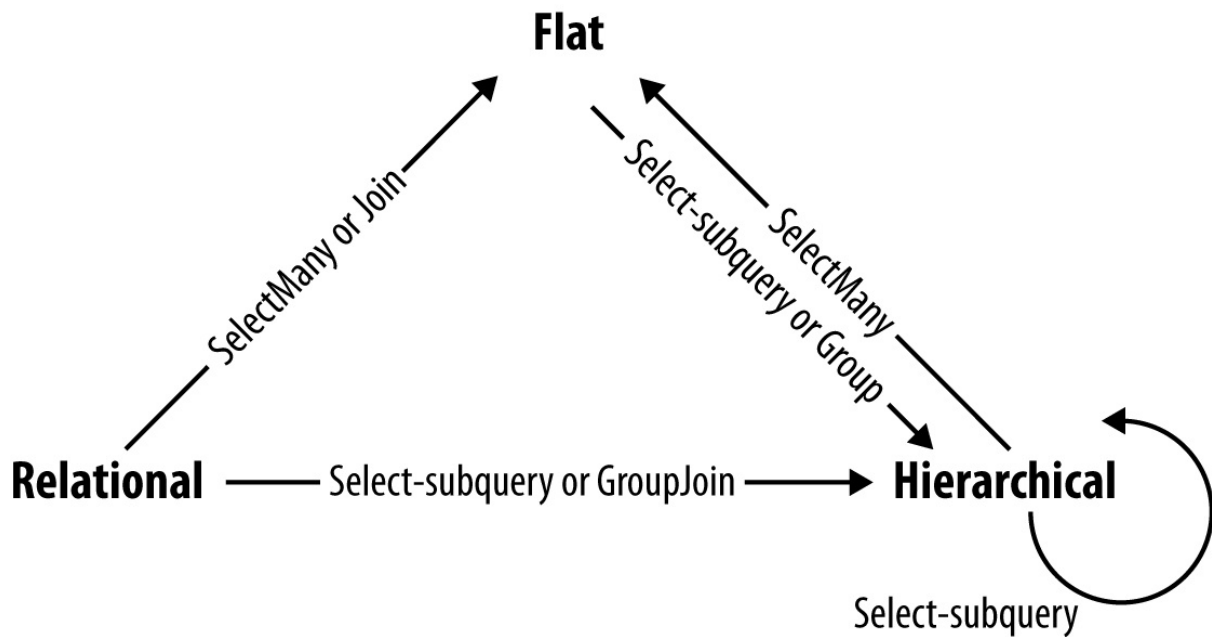
Figure 9-1. Shape-changing operators
