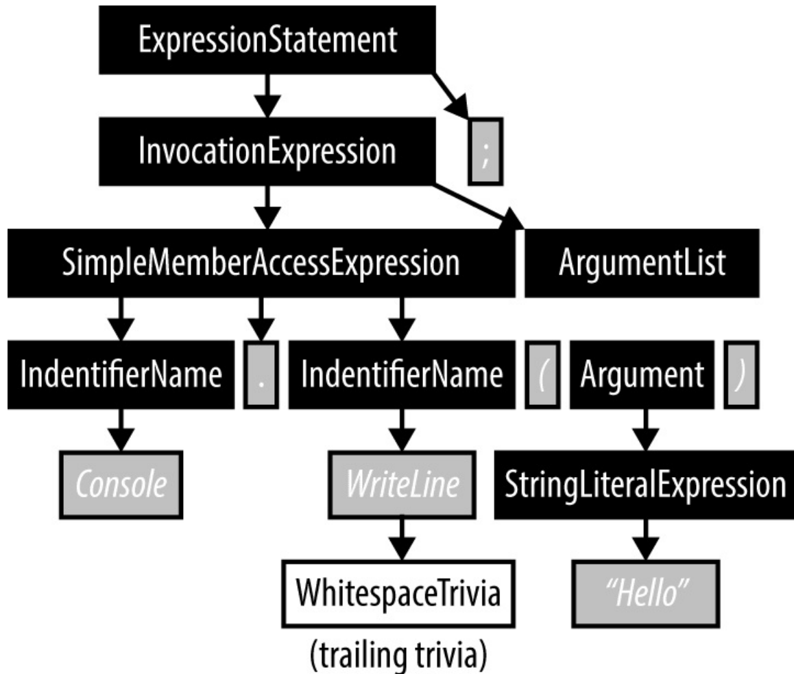
Figure 27-1. Syntax trees
