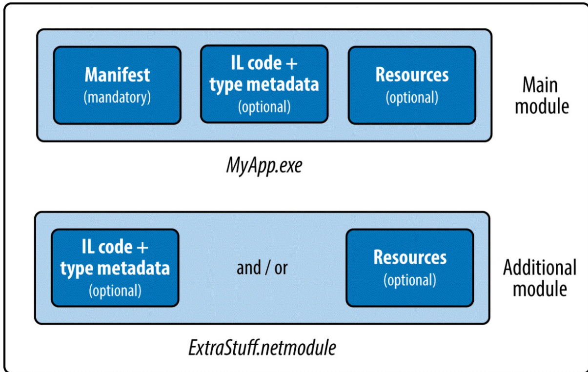
Figure 18-2. Multifile assembly
