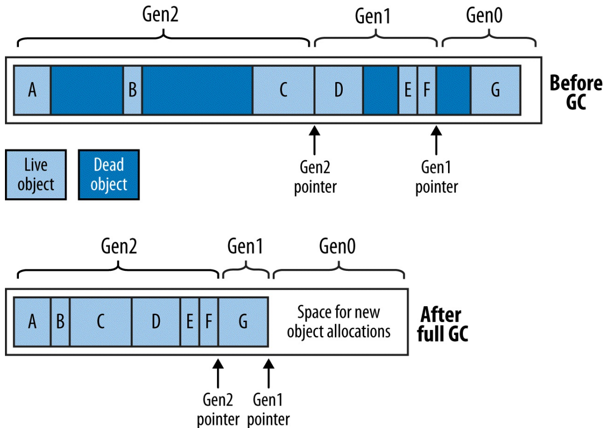
Figure 12-2. Heap generations
