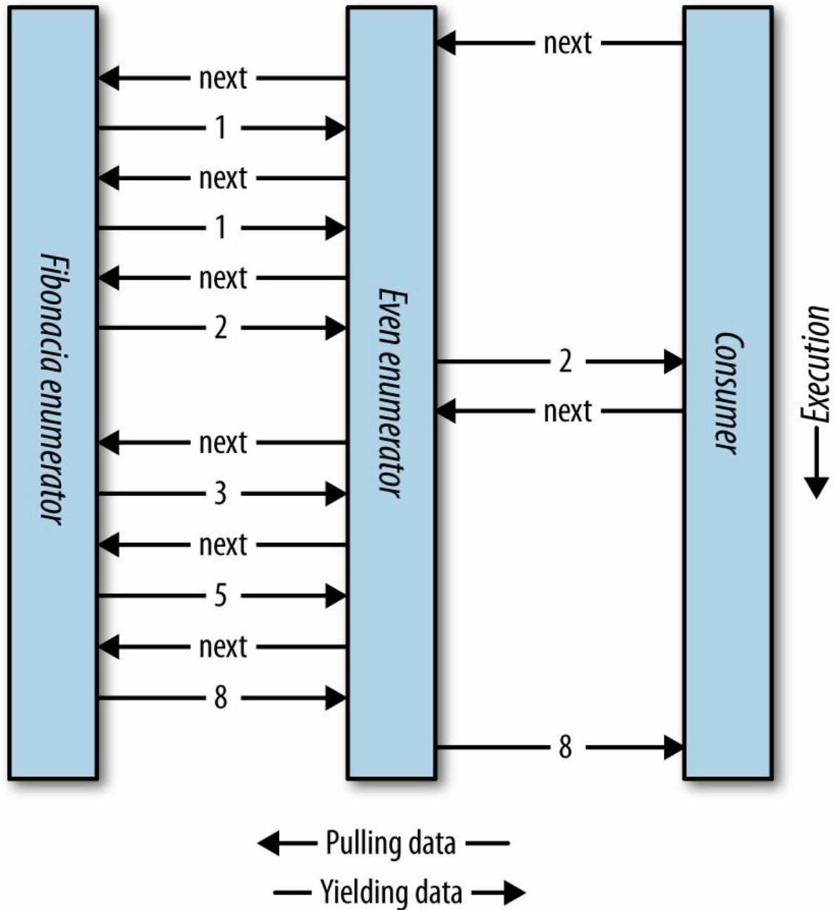
Figure 4-1. Composing sequences
