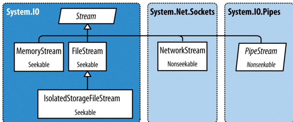
Figure 15-2. Backing store streams
