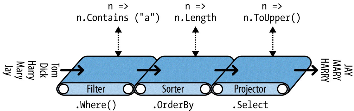
Figure 8-1. Chaining query operators
