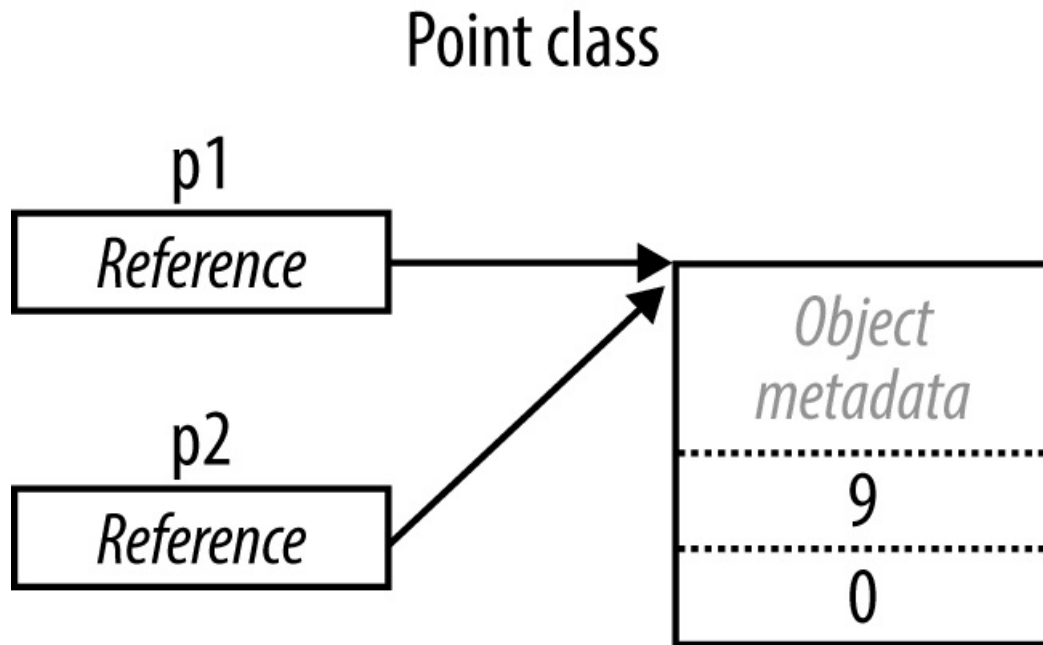
Figure 2-4. Assignment copies a reference
