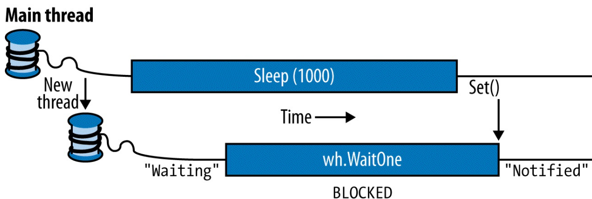
Figure 22-1. Signaling with an EventWaitHandle
