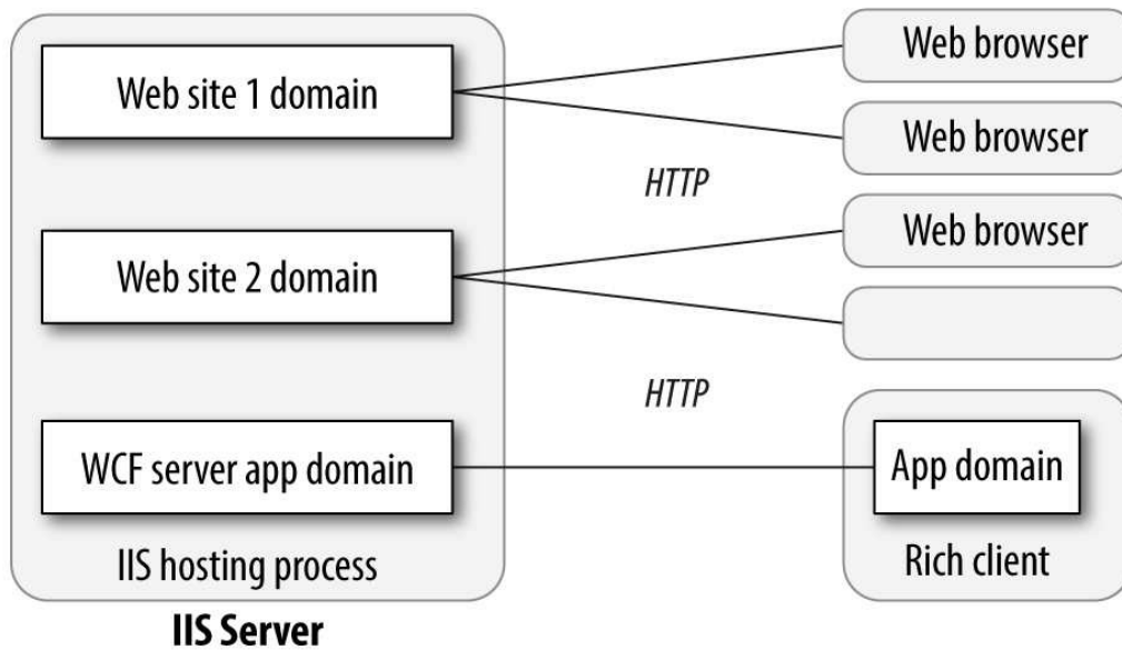
Figure 24-1. Application domain architecture
