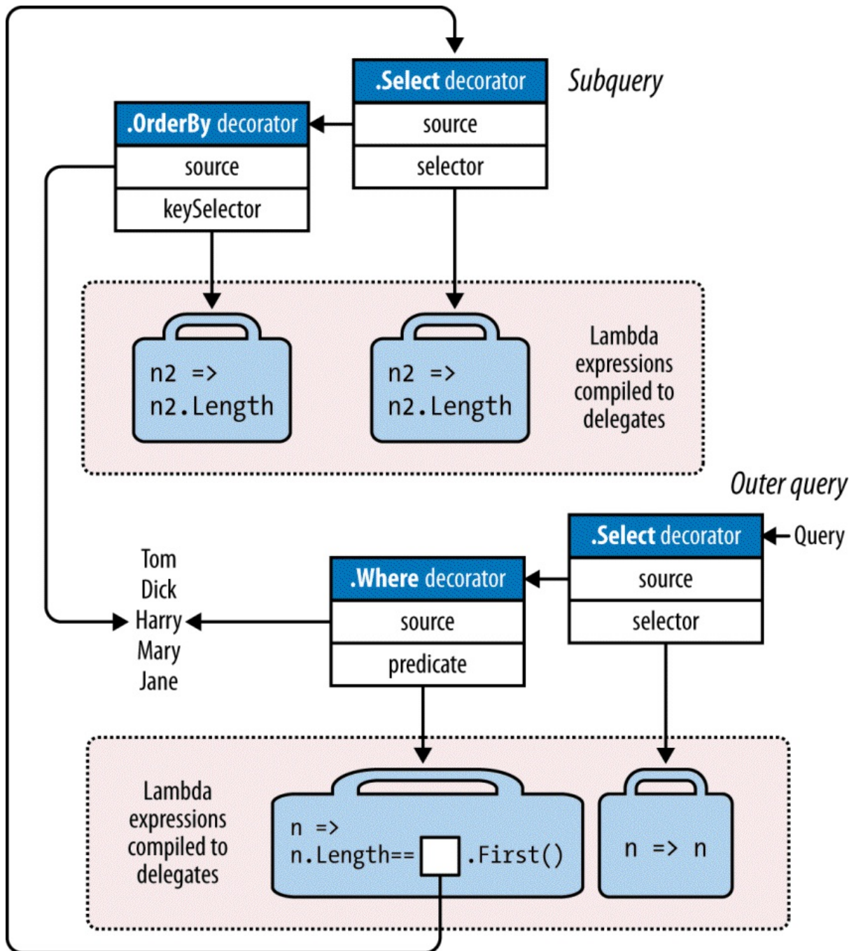
Figure 8-8. UML subquery composition
