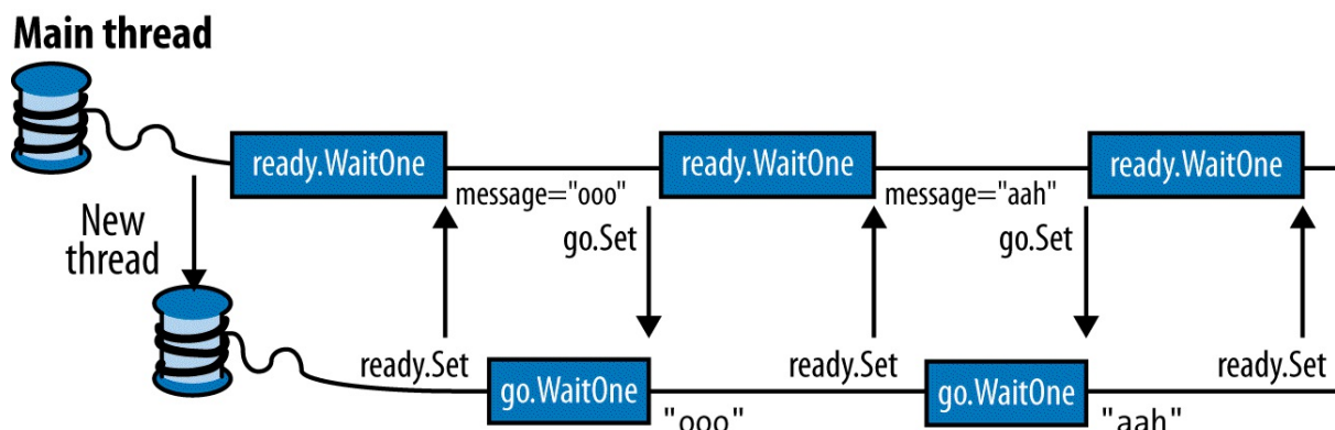
Figure 22-2. Two-way signaling
