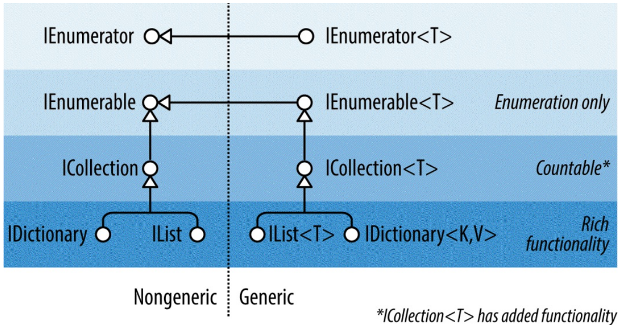
Figure 7-1. Collection interfaces
