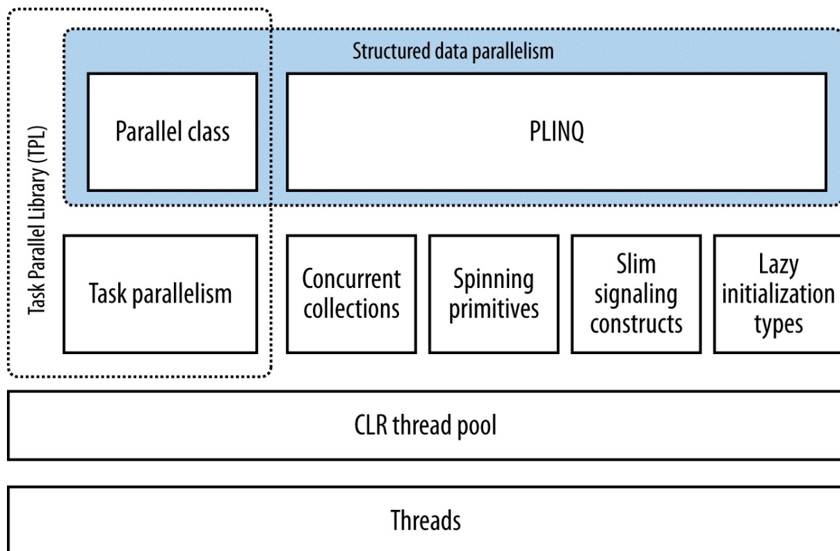
Figure 23-1. PFX components
