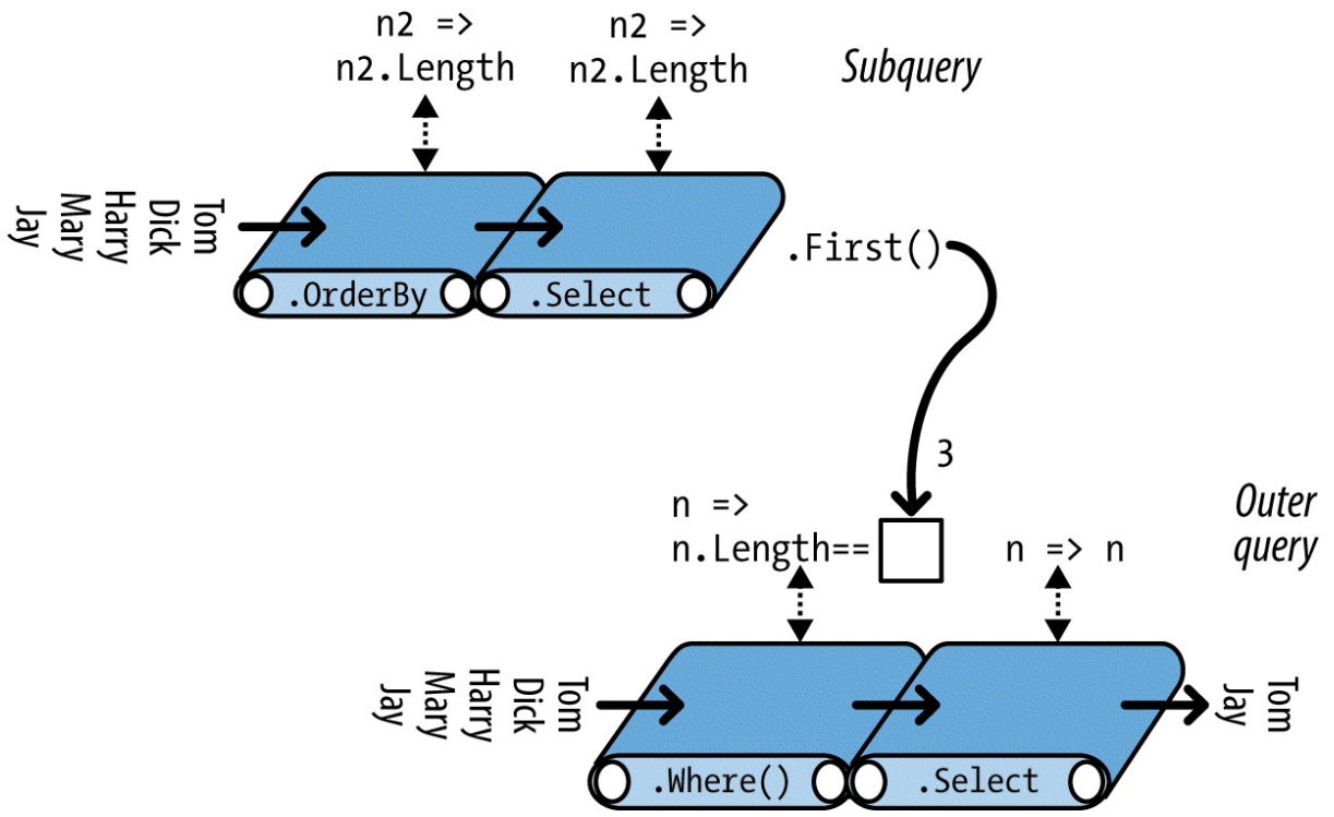
Figure 8-7. Subquery composition
