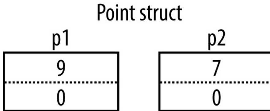
Figure 2-2. Assignment copies a value-type instance
