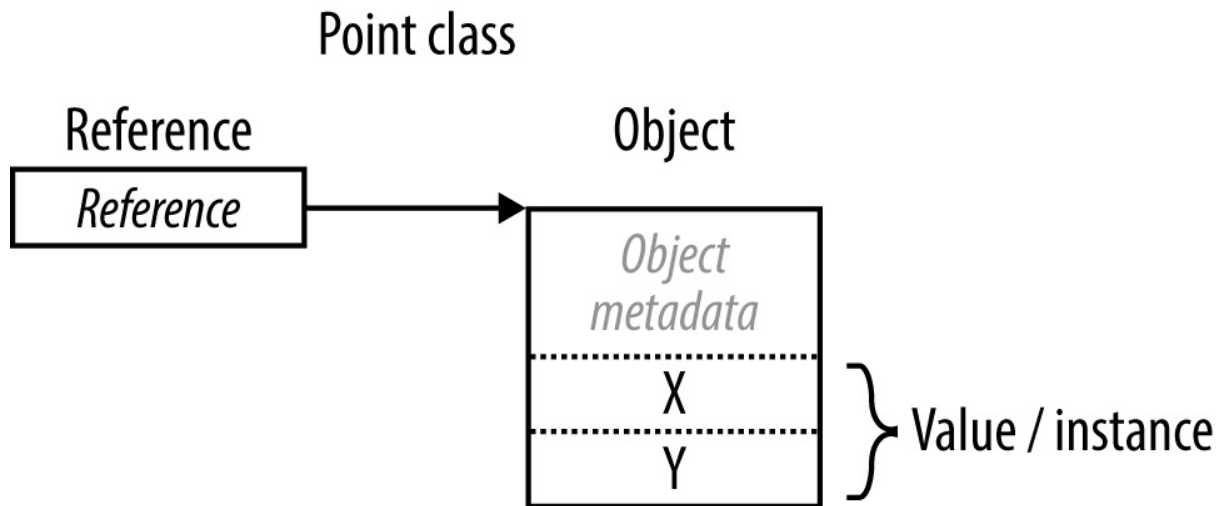
Figure 2-3. A reference-type instance in memory
